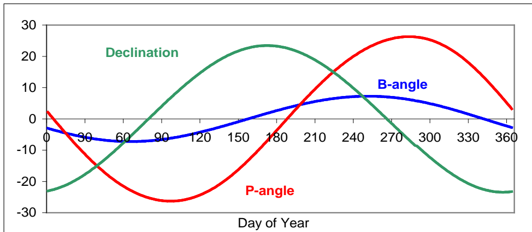
Figure 6. Yearly variation of B_0 , P, and solar declination \delta . Historically, P-angles for the sun are signed and lie in [-180:+180] , rather than in the usual [0:360] .
